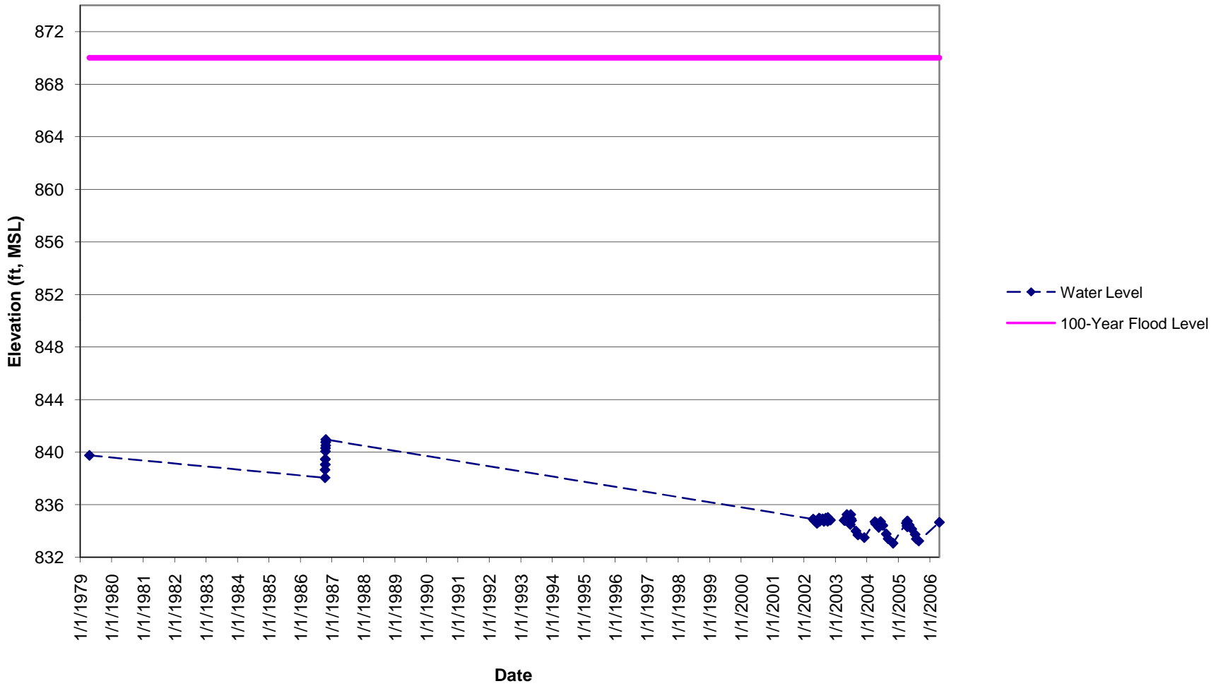
FAHLSTROM POND WATER LEVELS Valley Branch Waterhsed District
