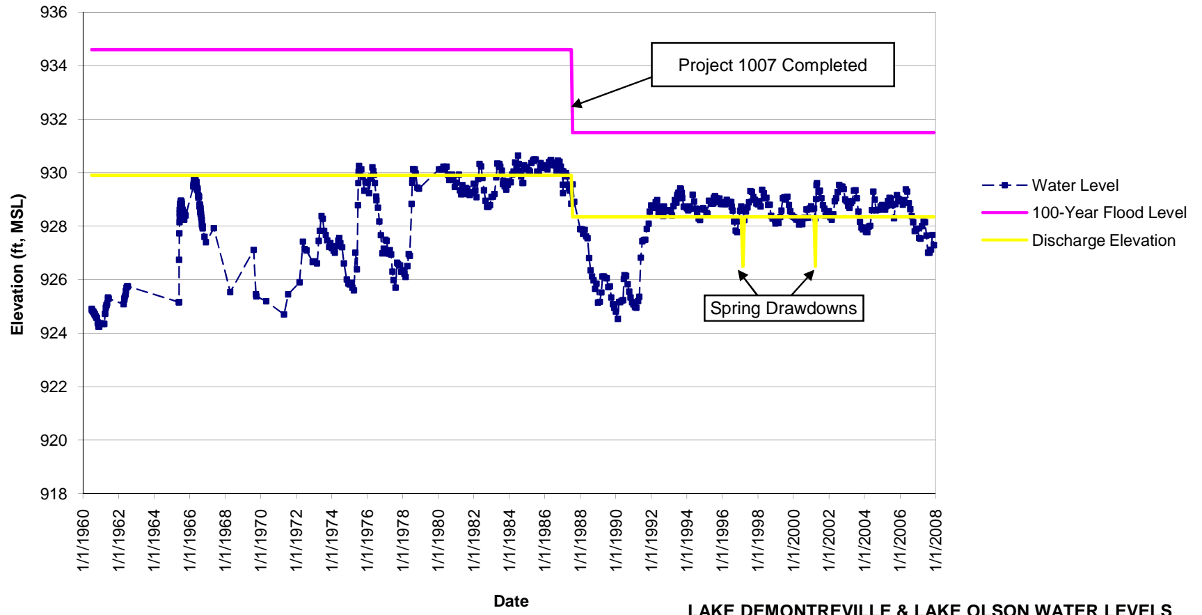
LAKE DEMONTREVILLE & LAKE OLSON WATER LEVELS Valley Branch Watershed District
